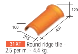
321 XT Residence ridge tile + clip - 2.5 per m. - 3.6 kg.
