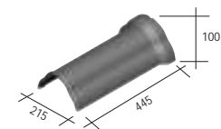
321 XT Residence ridge tile + clip - 2.5 per m. - 3.6 kg.
