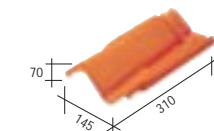
5 P8 1/2 tile - 1.8 kg.
