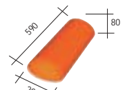
45 XG Languedocienne barrel hip end - 3.5 kg.
