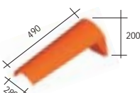
41 XG Barrel ridge starter for non interlocking ridge 500 mm - 5.4 kg.
