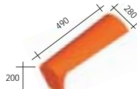
42 XG Barrel ridge end for non interlocking ridge 500 mm - 5.8 kg.
