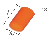
452 XG Circular ridge hip end 400 mm - 4.6 kg.
