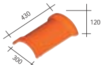
31 XG Interlocking ridge with collar - 2.5 per m. - 4.1 kg.
