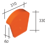
36 XG Interlocking collar ridge end (pediment) - 2.5 kg.
