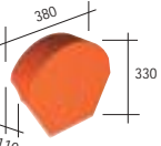
351 XG Universal tubular ridge end (pediment) - 3.2 kg.
